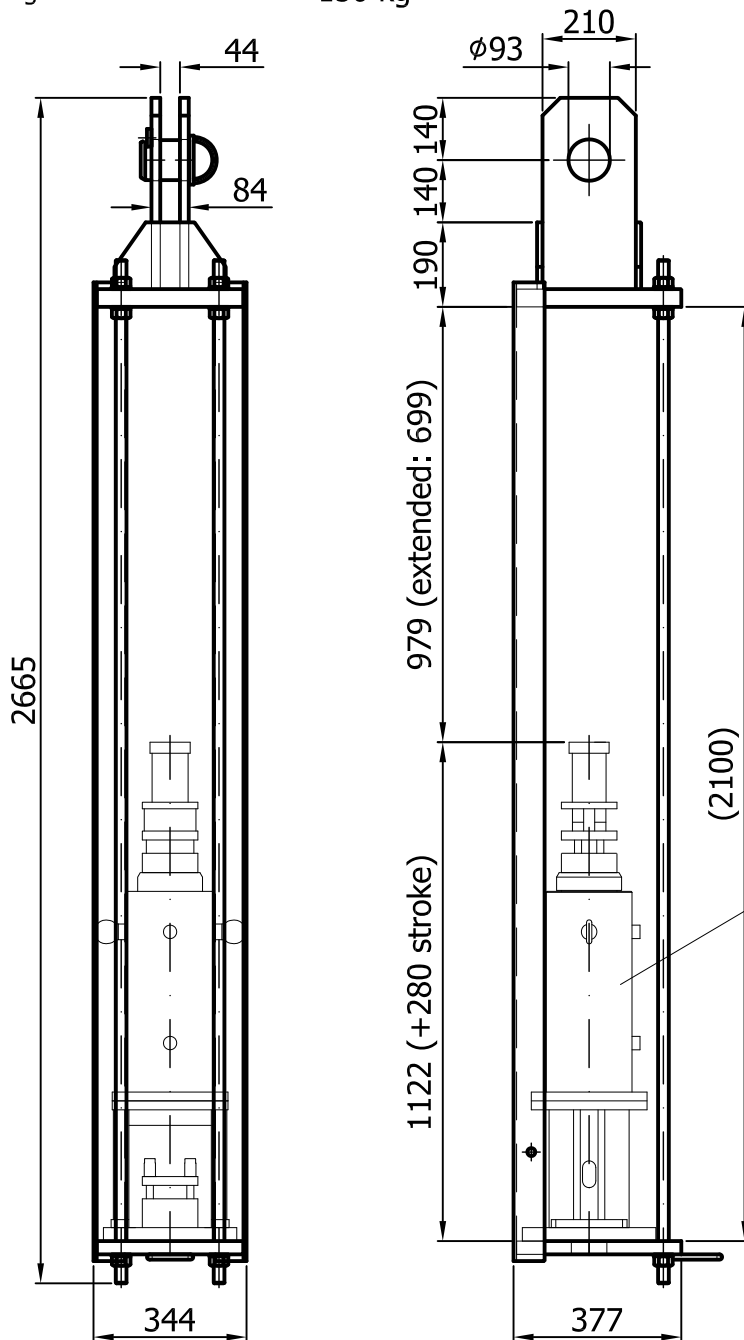
Strandjack H-40
